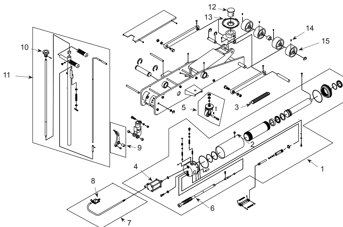
Figure 2 — Repair Parts Illustration
