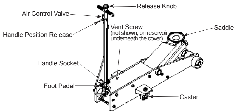
Figure 1 — Hydraulic Service Jack Components
