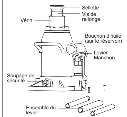
FIGURE 1 - Cric-bouteille type
