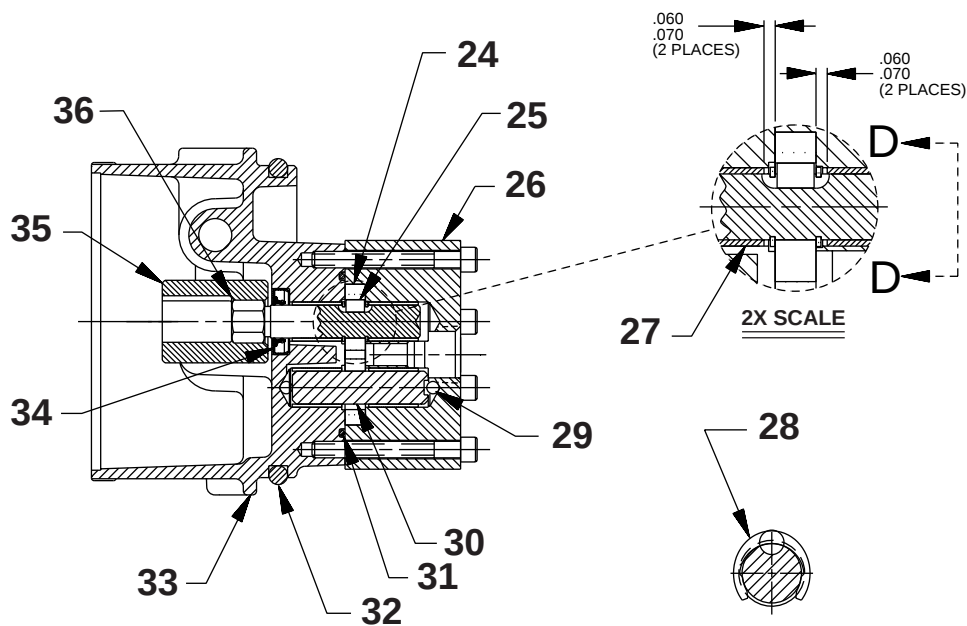
VIEW D-D 2X SCALE
