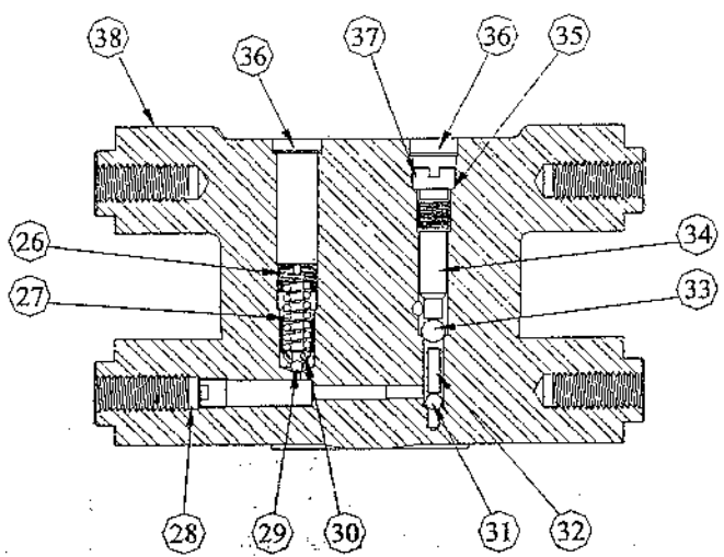
"HYDRAULIC UNIT BASE CROSS SECTION"
