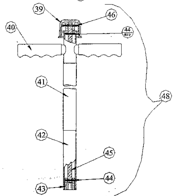
"T-HANDLE CROSS SECTION"
