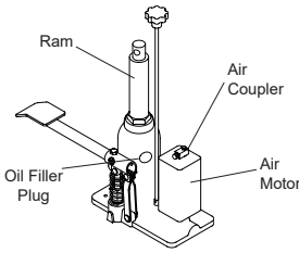
Air Operated Hydraulic Unit
