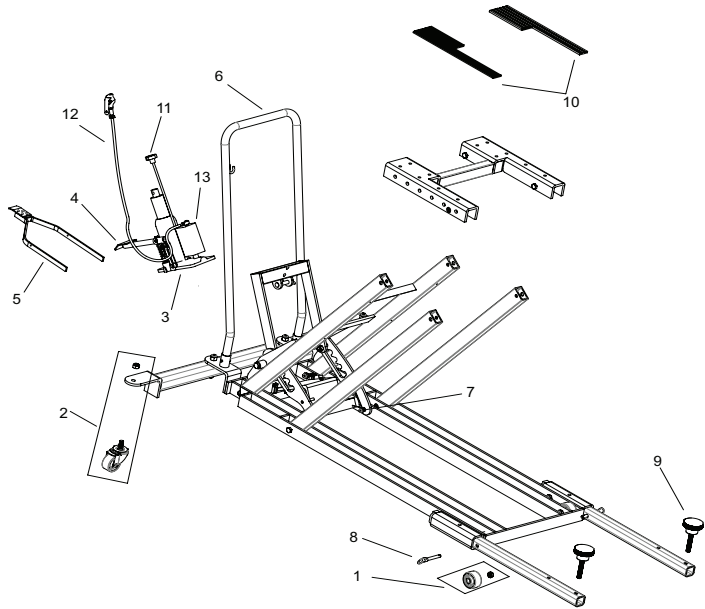
Figure 5 - Replacement Parts Illustration for Model T-1250
