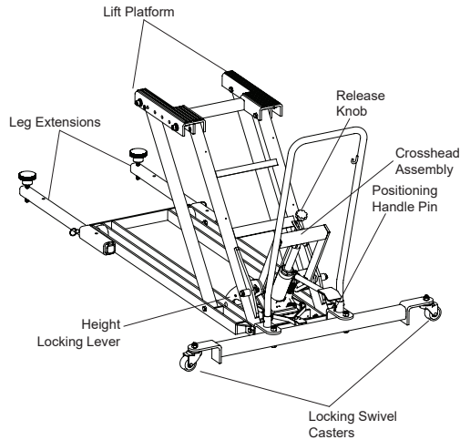
Figure 1 - Model T-1250 Nomenclature
