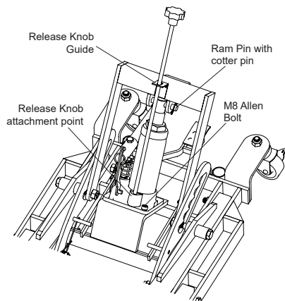
Figure 2 - Hydraulic Unit assembly
