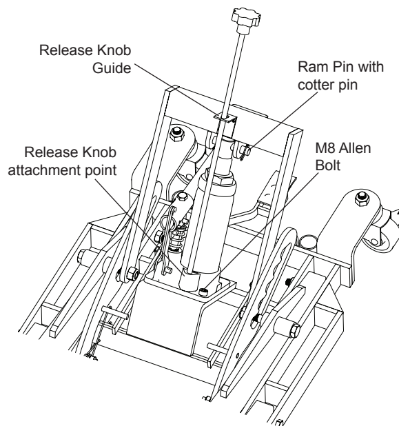
Figure 2 - Hydraulic Unit assembly
