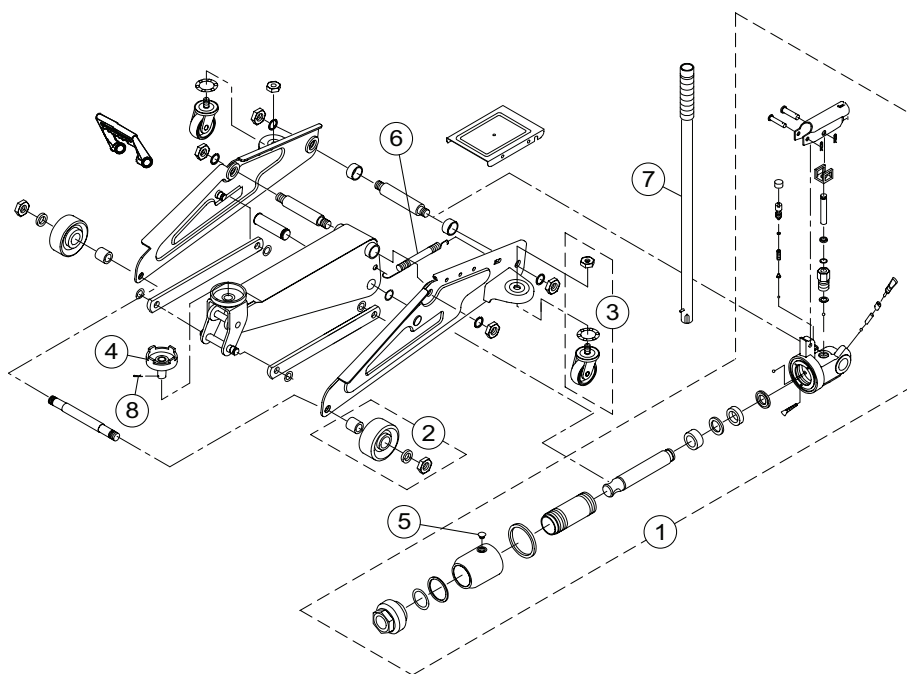
Figure 3 - Replacement Parts Illustration
