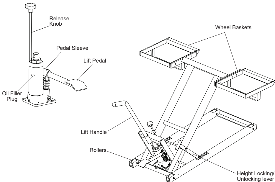
Mower Lift Nomenclature
