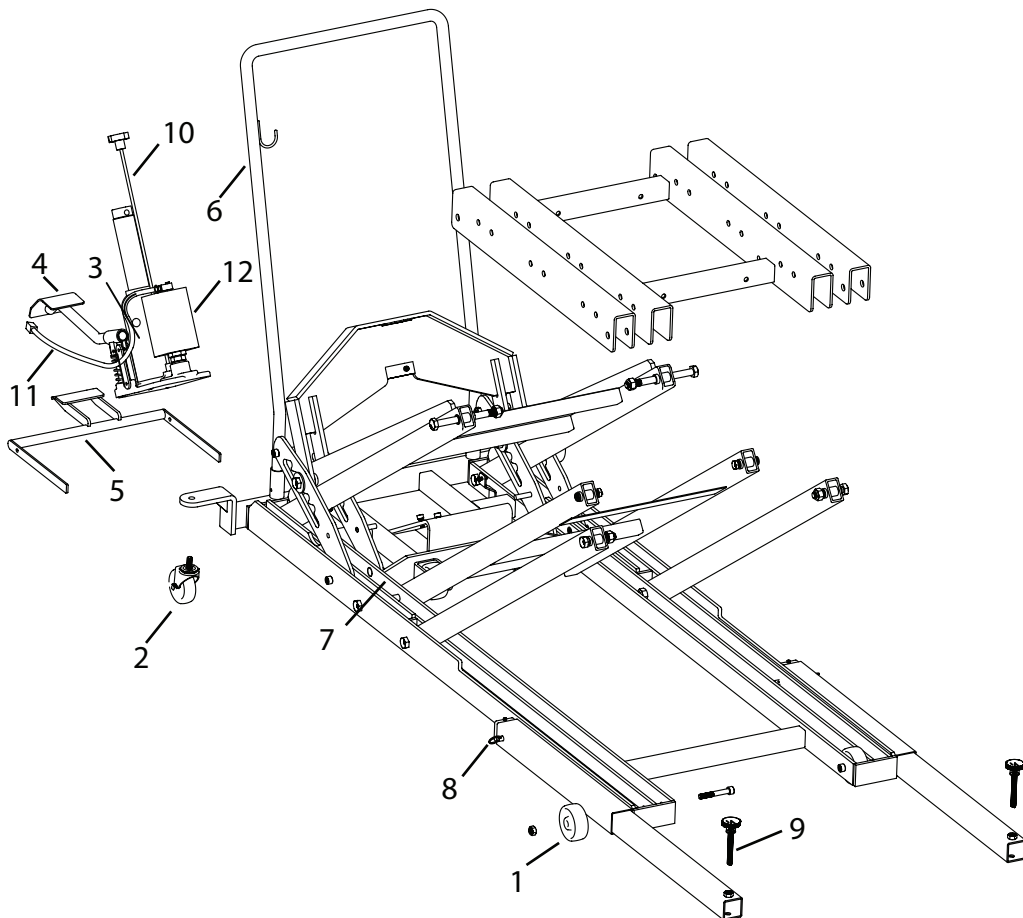
Figure 5 - Replacement Parts Illustration for Model 2830425
