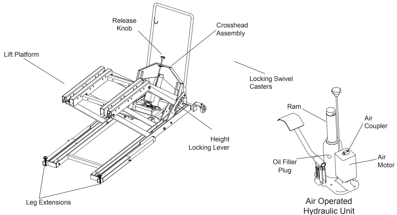
Figure 1 - Model 2830425 Nomenclature
