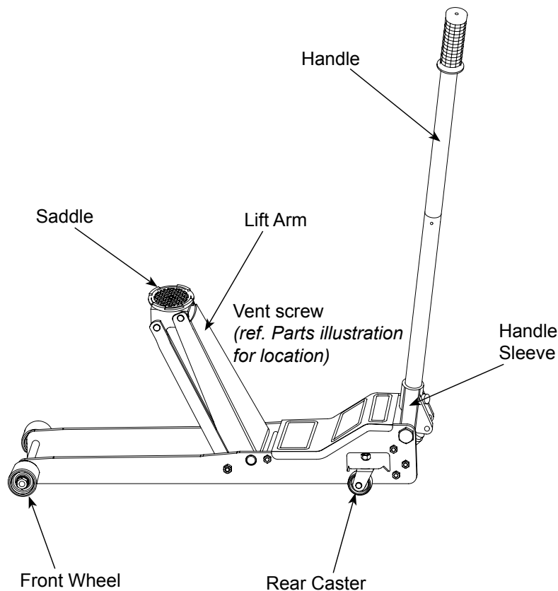
Figure 1 - Service Jack Nomenclature
