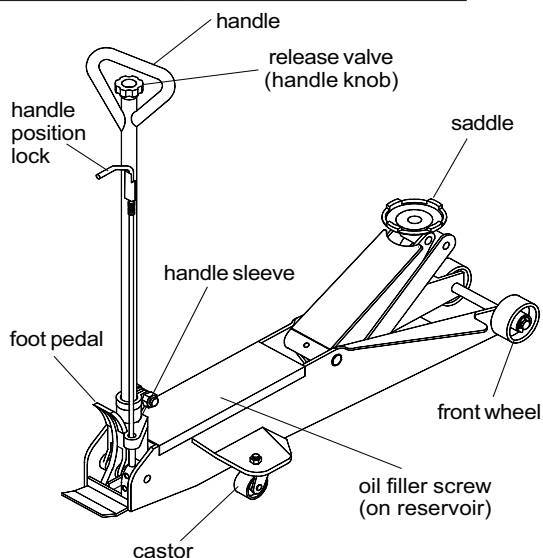
Figure 2 - Model 25057 & 25107 Components
