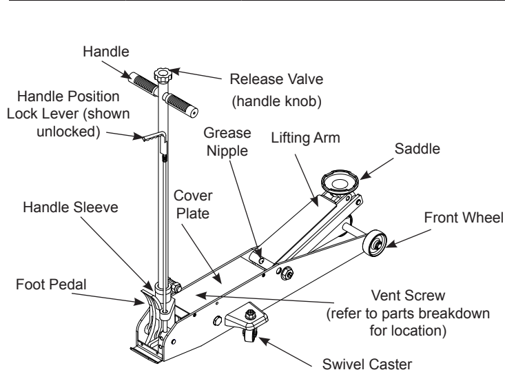
Figure 1 - Model 25048C Components
