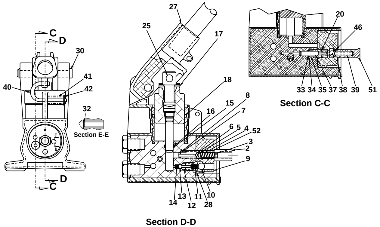
Figure 3. Section D-D
