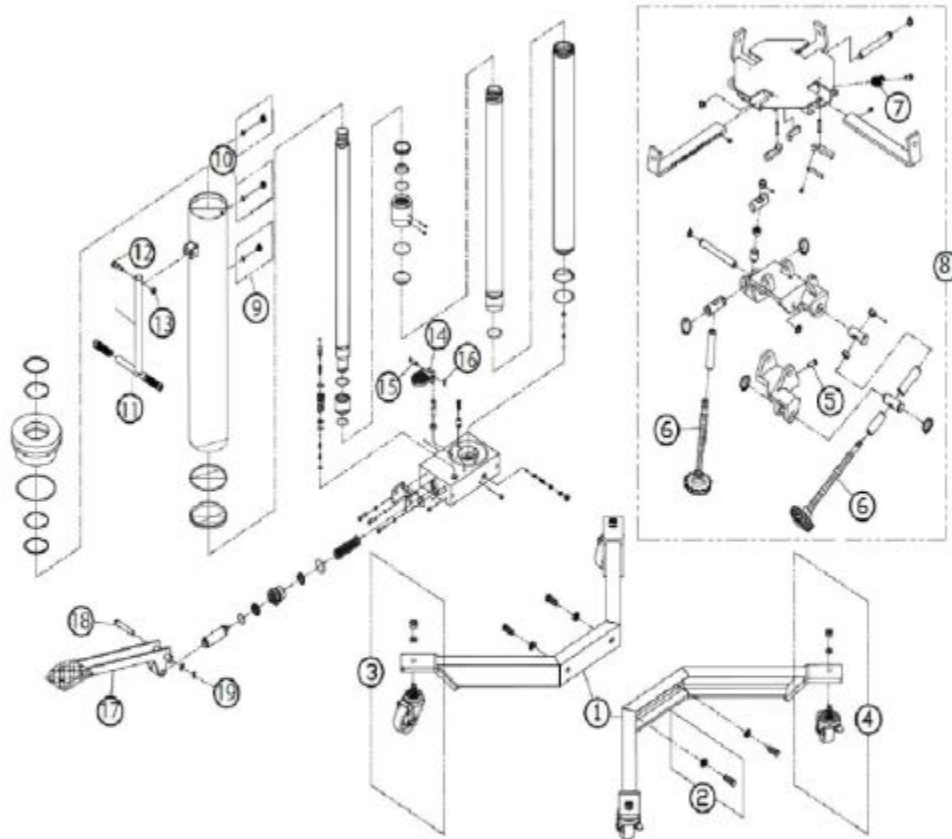
Figure 2 - Replacement Parts Illustration for Model TJ1000A Series A
