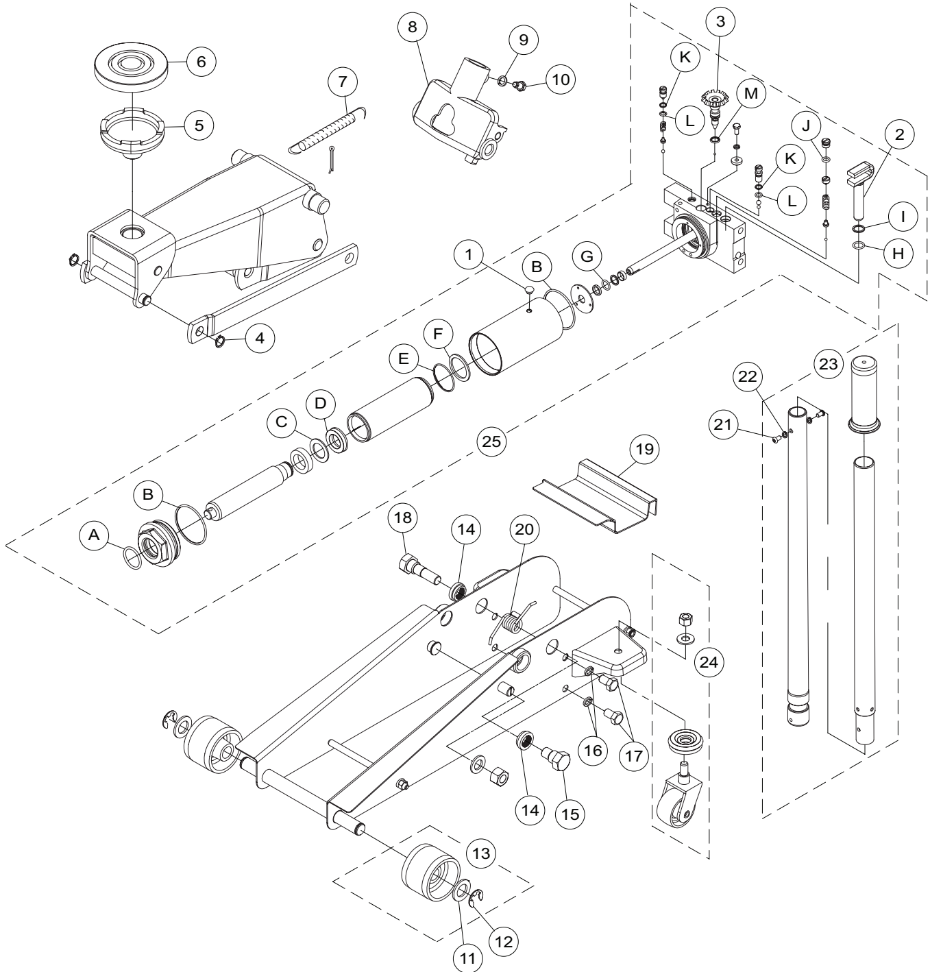
Figure 2 - Replacement Parts Illustration for Model MFJ3T
