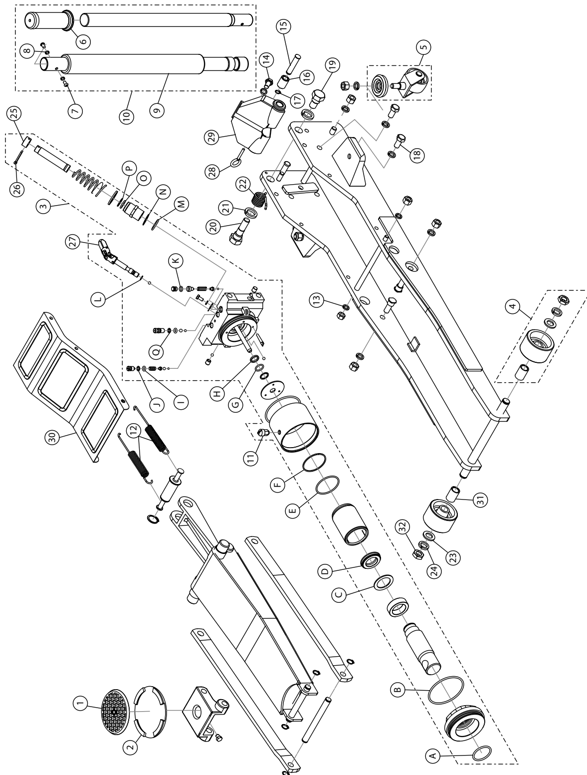
Figure 2 - Replacement Parts Illustration for Model LPSJ2T
