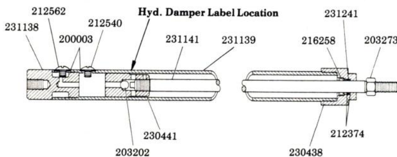
231136 HYDRAULIC DAMPER
