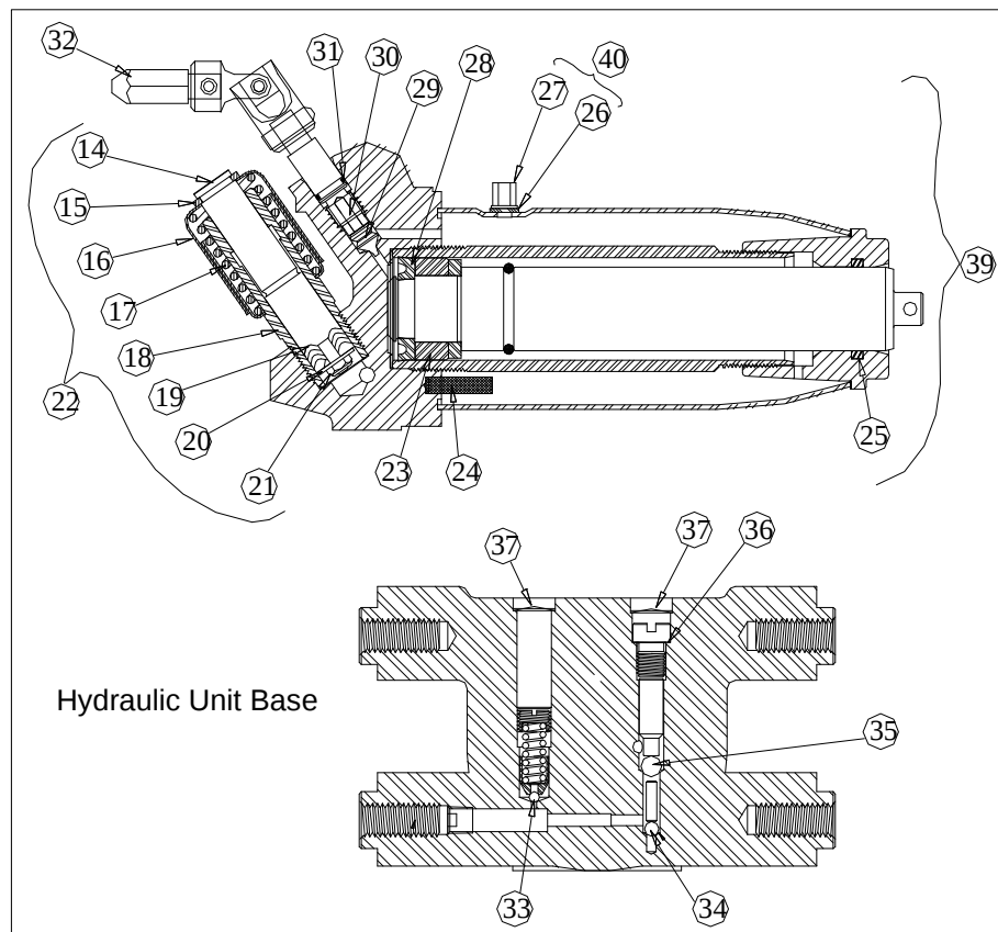
Figure 2: Parts Illustration for FSJ-40B and FSJ-60B QUICKLIFT®
