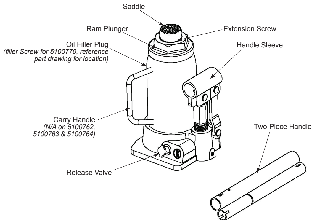
Figure 1 - Typical Bottle Jack Nomenclature (5100768 shown)
