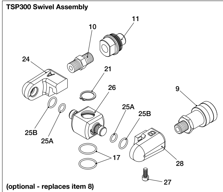
Figure 3, Drive Unit and Swivel Assembly, W35000X Series
