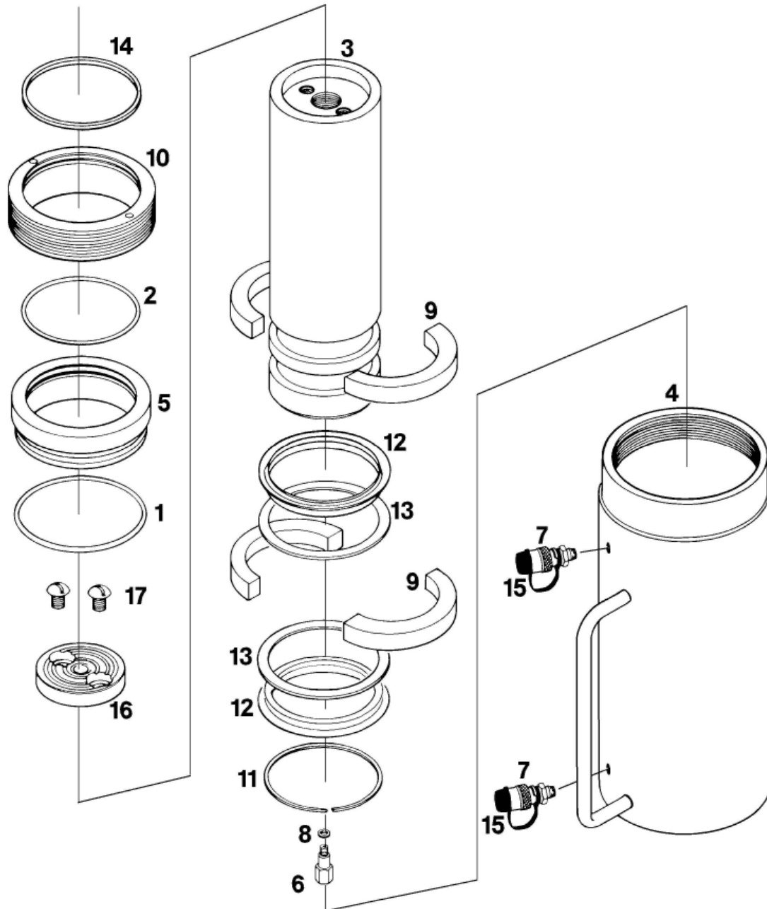
75 Ton 6" Stroke Double-Acting Hydraulic Cylinder
