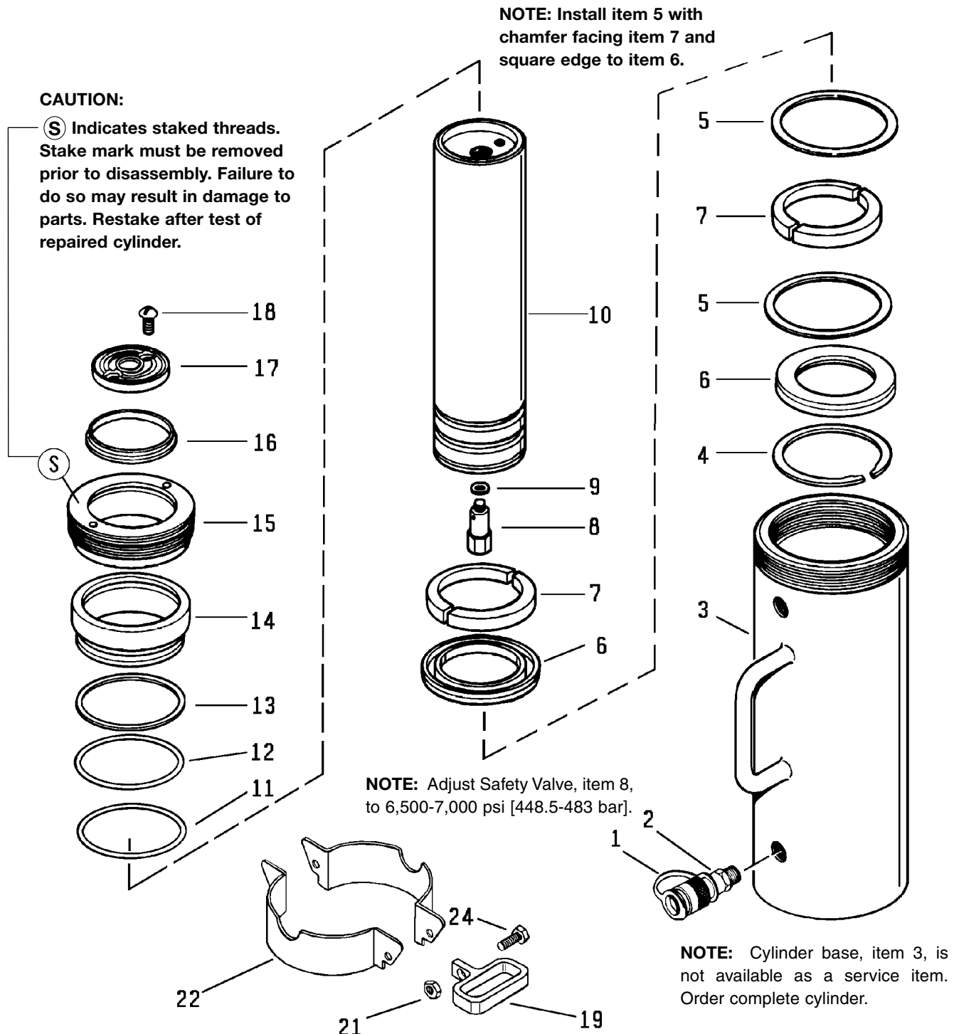
Figure 1, 50-Ton Double-Acting Solid Plunger Hydraulic Cylinder
