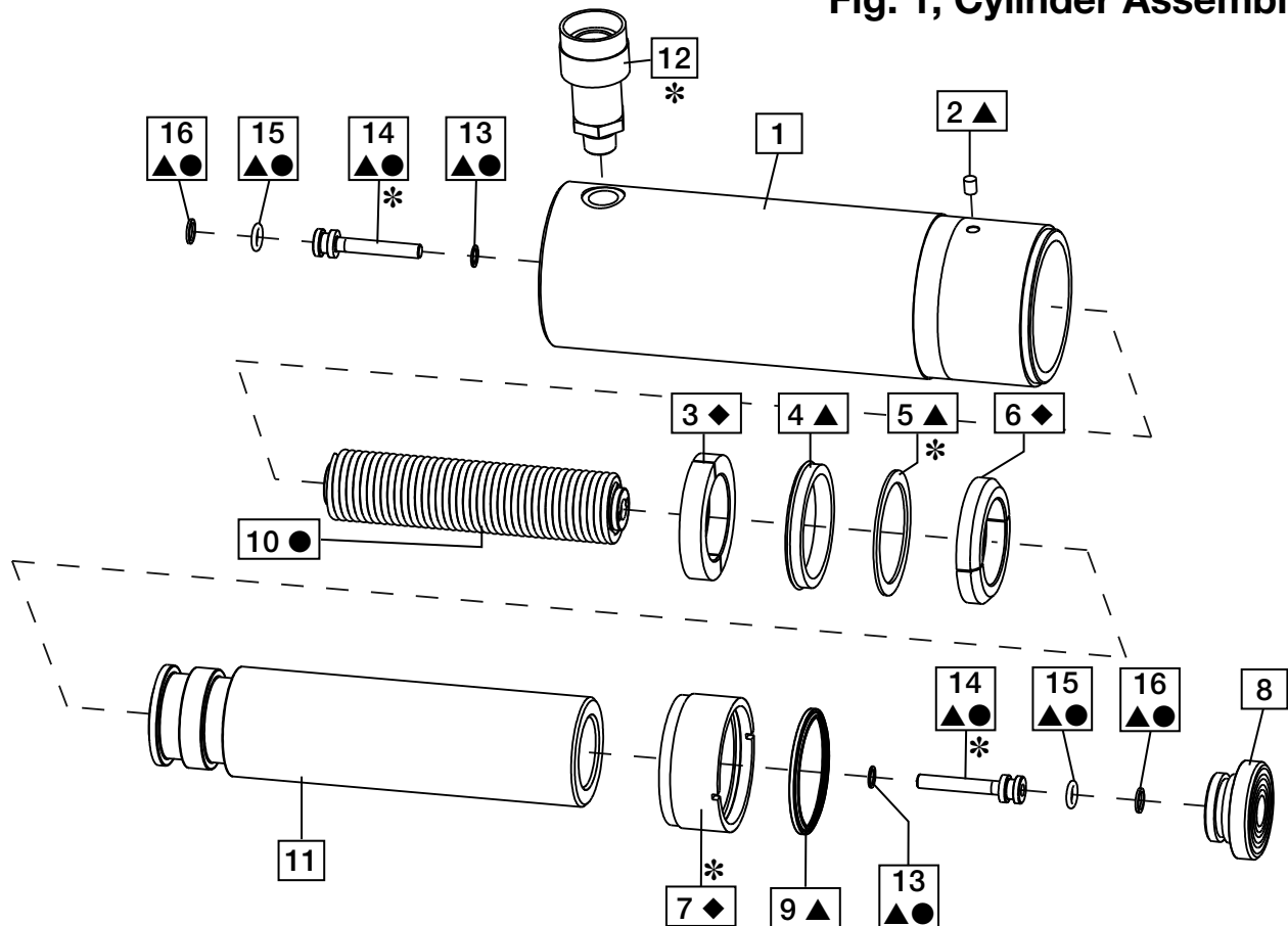
Fig. 1, Cylinder Assembly
