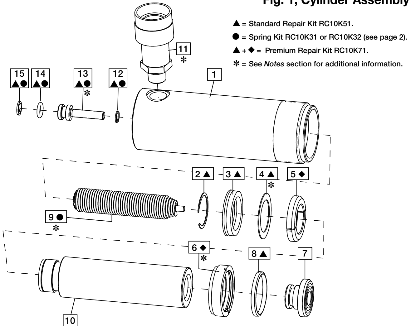
Fig. 1, Cylinder Assembly
