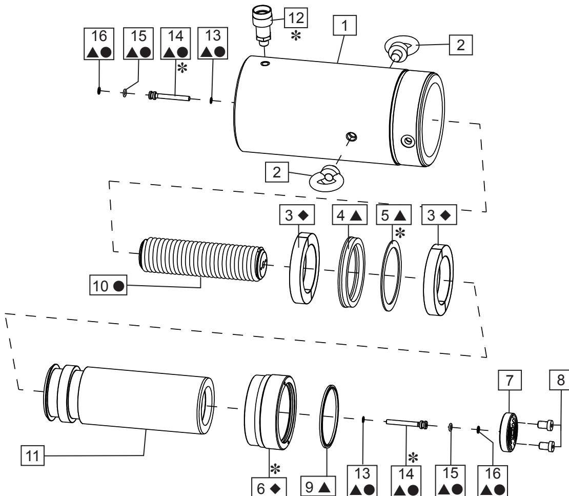
Fig. 1, Cylinder Assembly
