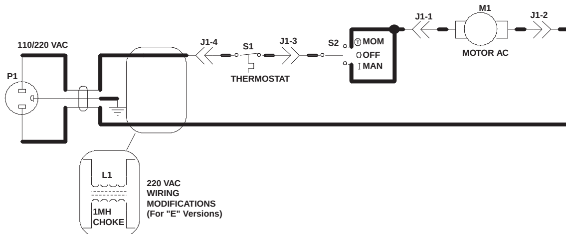
Figure 2: Wiring Diagrams.
