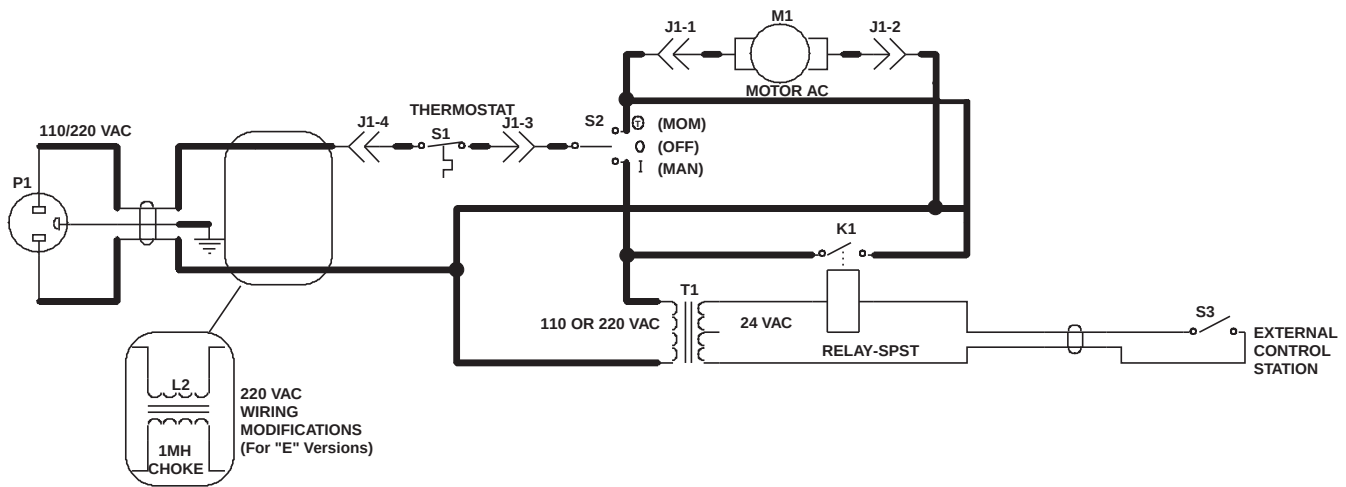
Figure 4: Electrical Schematic for PUJ Models.
