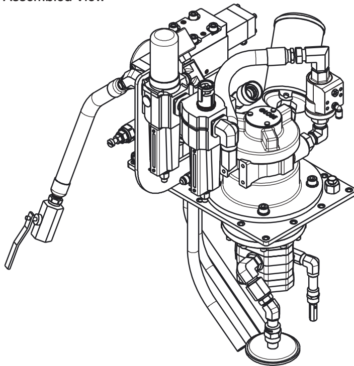
Assembled View
