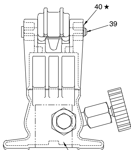
Fig. 4, Front View
