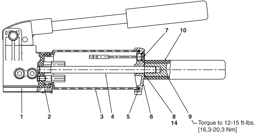
Figure 1, Pump Assembly
