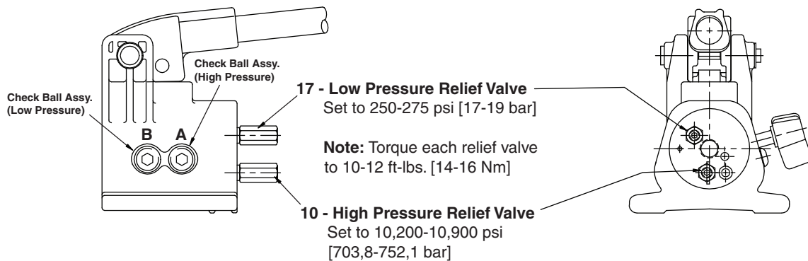
Figure 2, Pumping Unit Assembly (See parts list on page 2)
