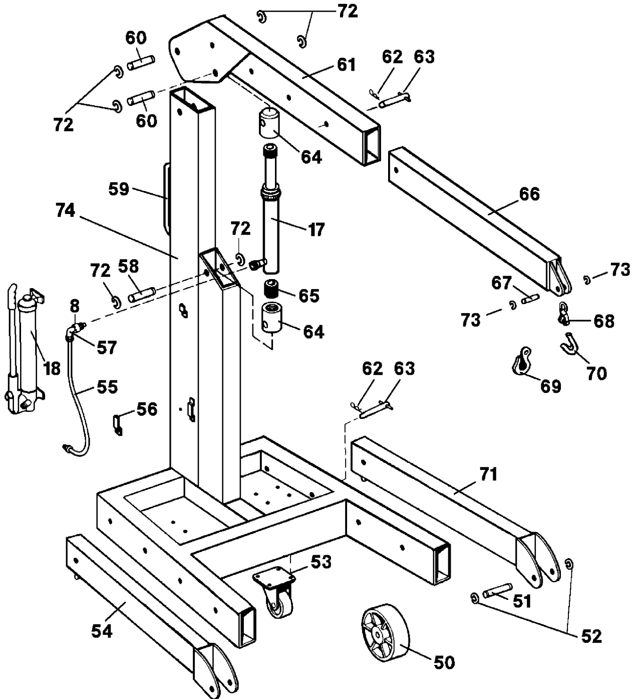
MOBILE CRANE UNIT PARTS DRAWING (ITEMS 50-74)
