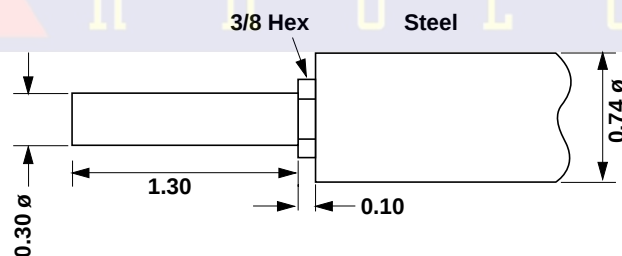
Figure 6 - 3,000 psi Tool
