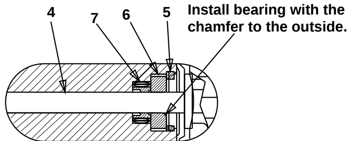
Detail D
