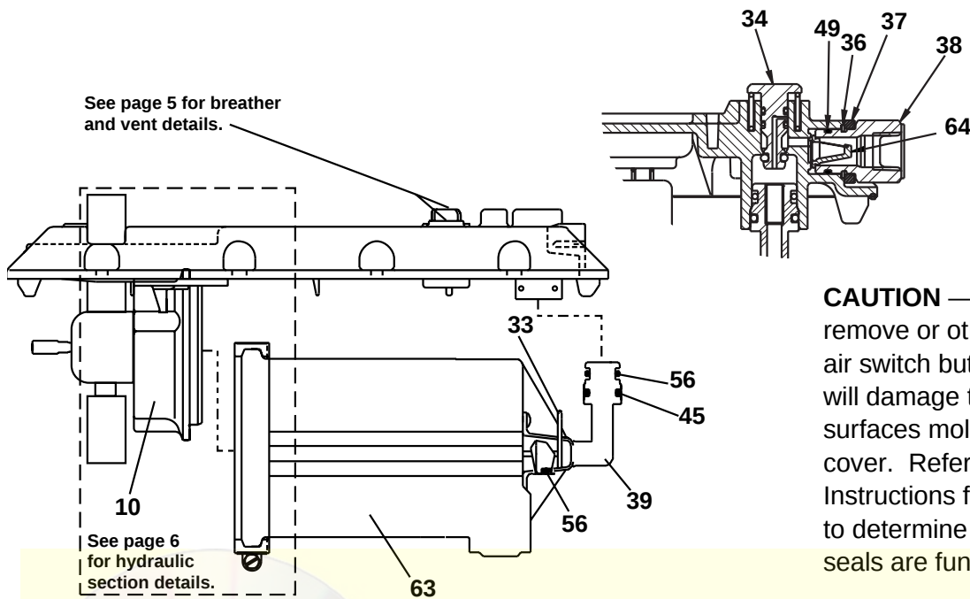
Figure 2 - Cover Assembly Side View
