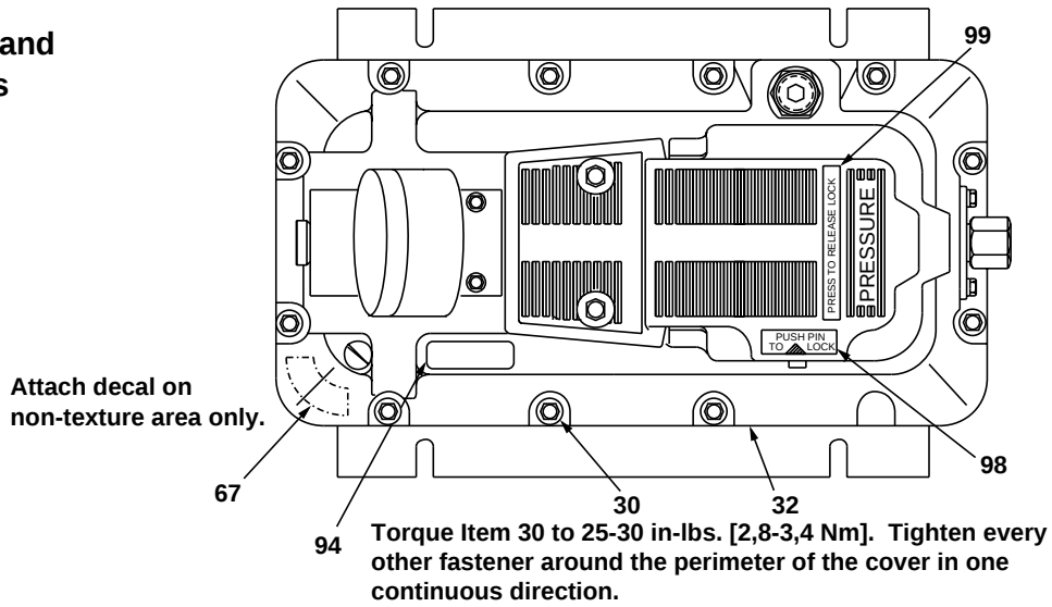
Figure 1 - Reservoir Cover & Treadle
