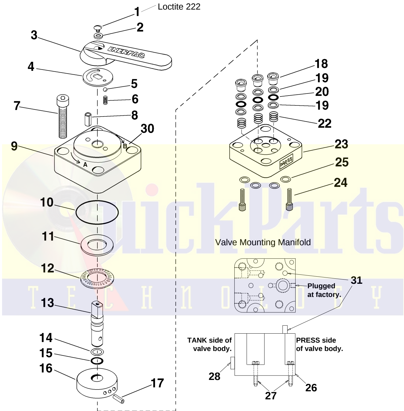
Figure 10 - Manual Valves (PAM Models)
