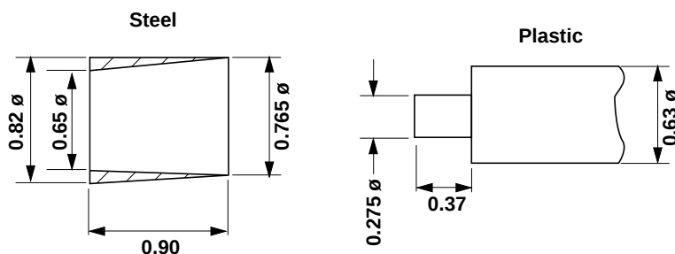
Figure 7 - 5,000 psi Tools
