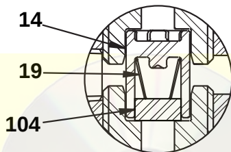
Detail E
