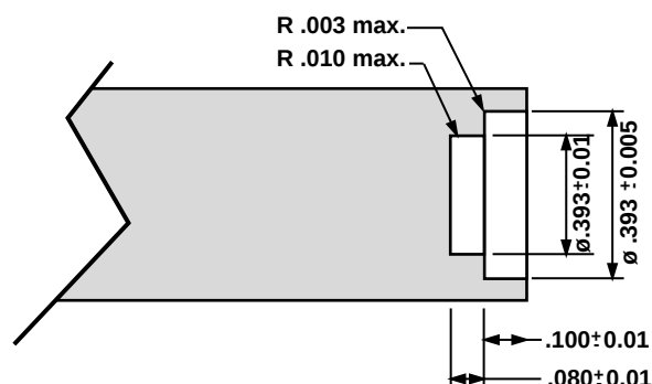
Figure 3 - Cover Assembly Tool
