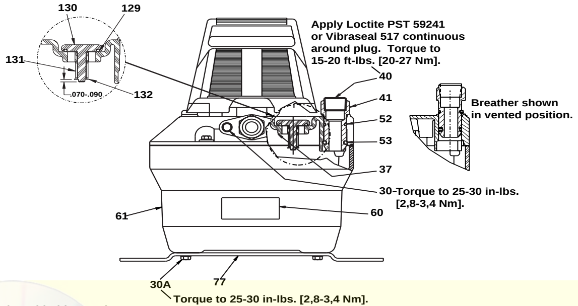
Figure 4 - Reservoir End View
