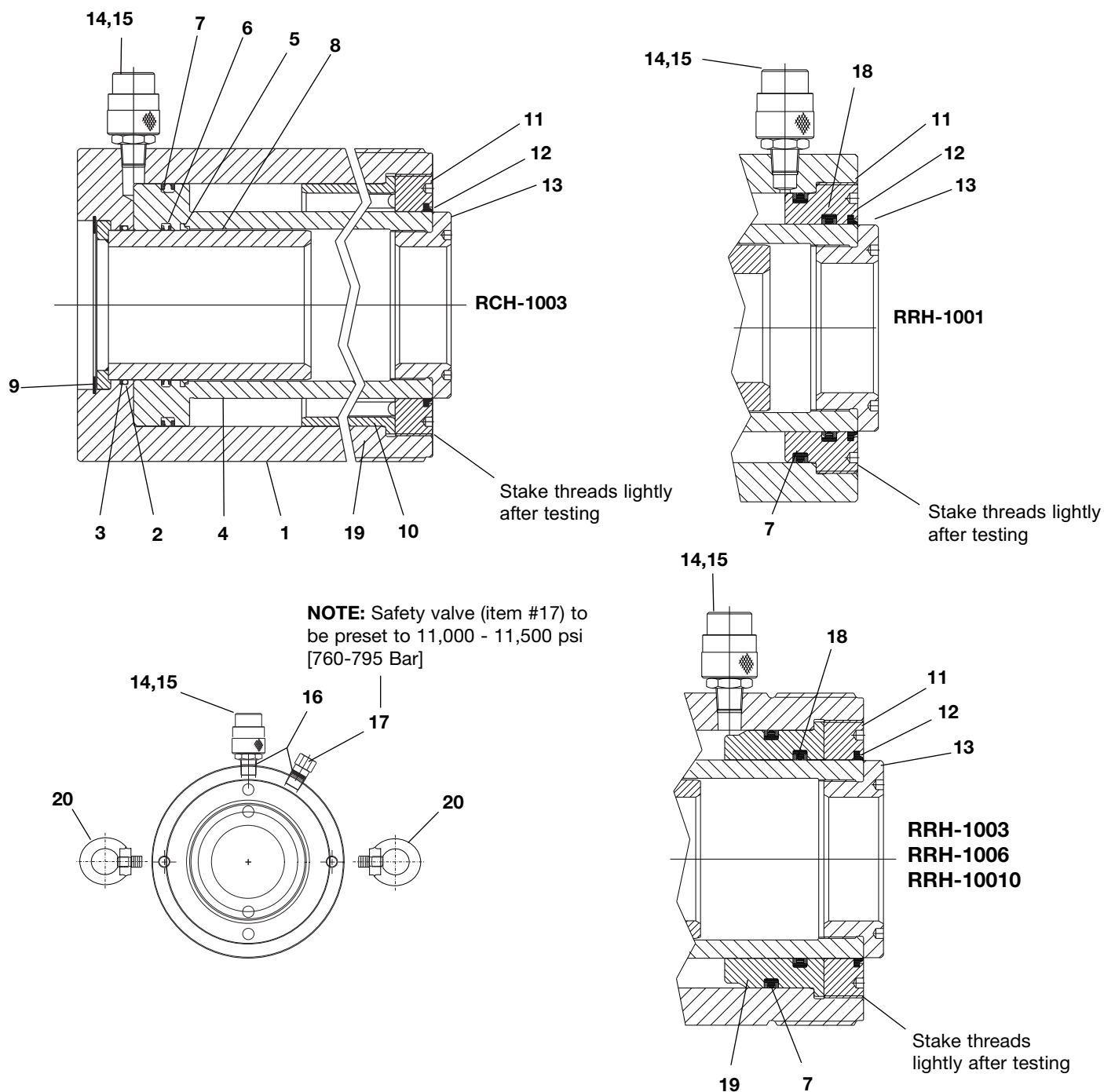
Figure 1, 100-Ton Hollow Cylinders
