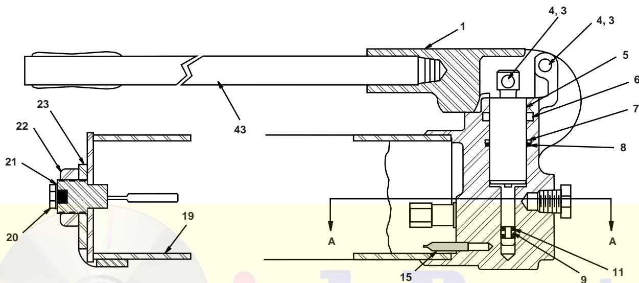
Figure 1, Pump Assembly
