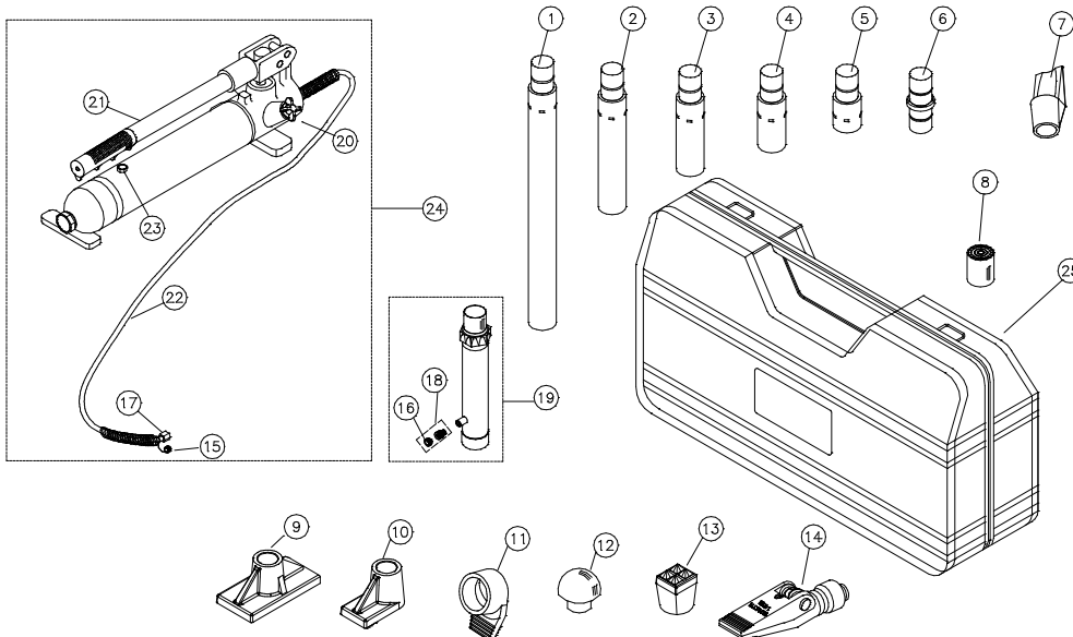
Figure 4 - Replacement Parts Illustration for Model 50364
