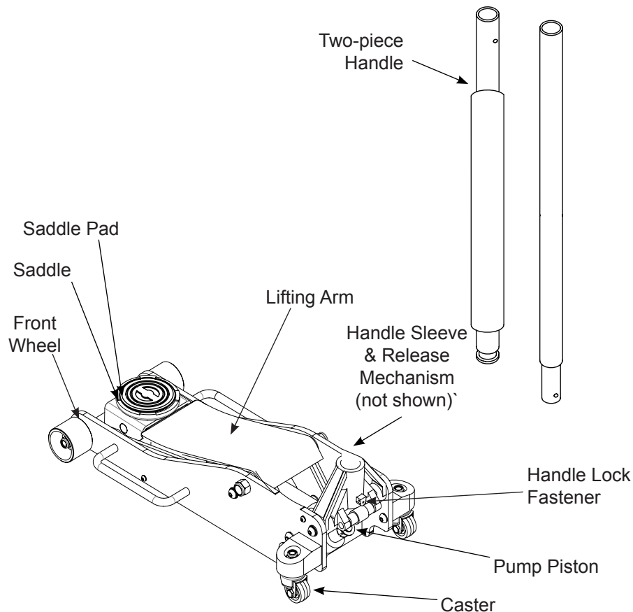
Figure 1 - Service Jack Nomenclature
