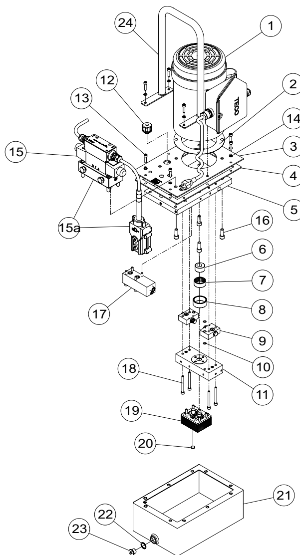
Fig. 2 PES0501T, PESM0501T Parts Illustration
