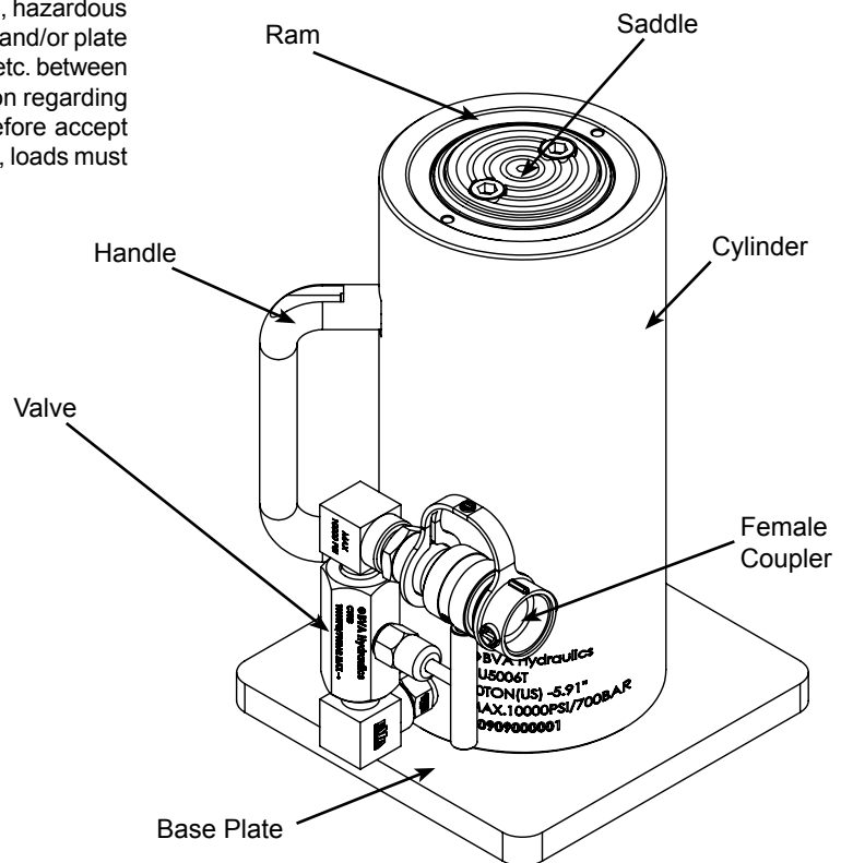
Figure 1 - Cylinder Components
