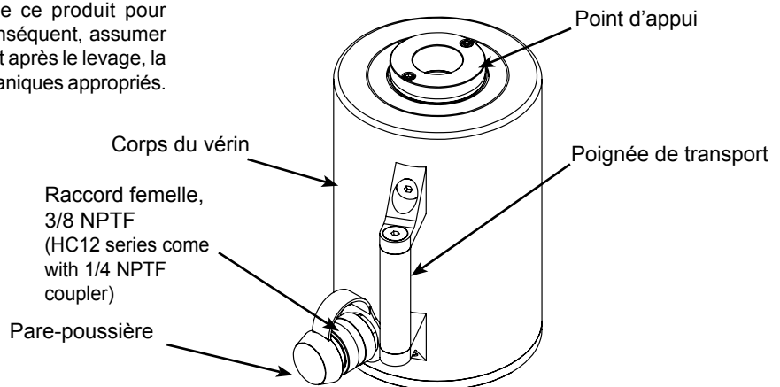
Figure 1 - Composants de vérin type
