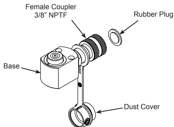
Figure 1 - Model H0500 Components
