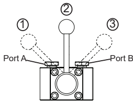
(a) 4-way, 3-position valve for Double Acting Cylinder
