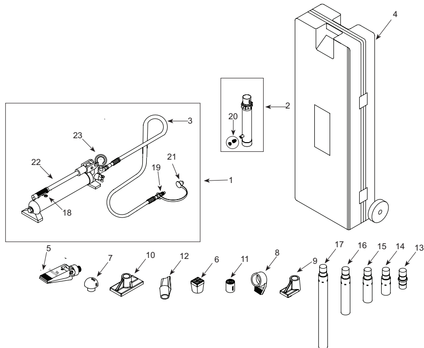
Figure 4 - Replacement Parts for Model YA1545
