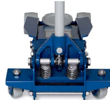
Rear View Showing Dual Pumps
