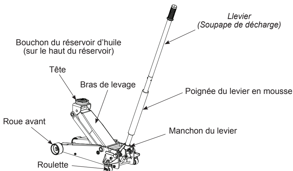
Figure 1 – Nomenclature typique de cric
