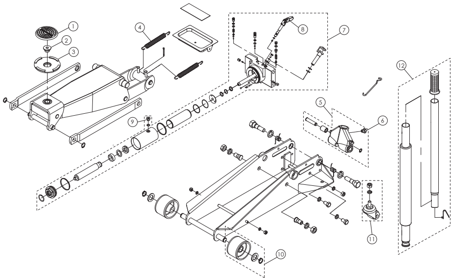
Figure 2 - Replacement Parts Illustration for Model B6350
