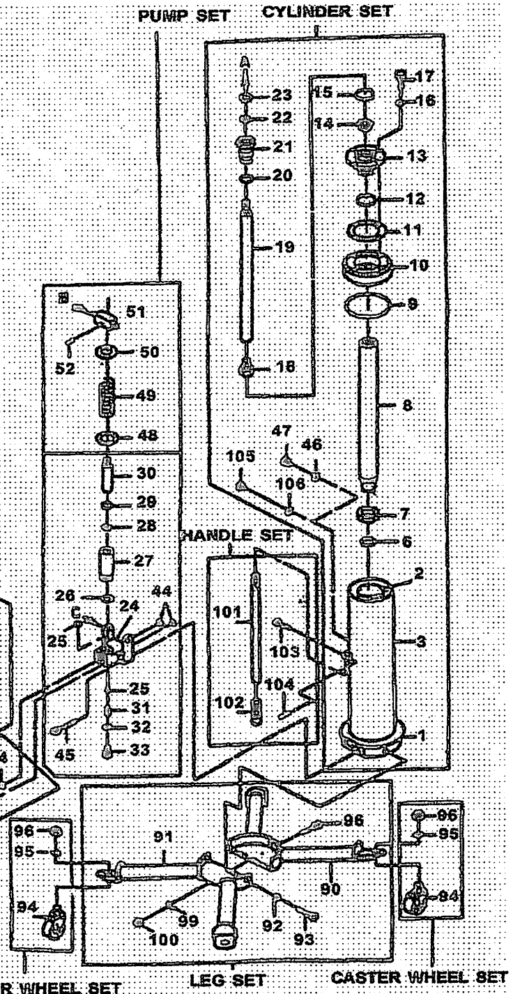
CASTER WHEEL SET
